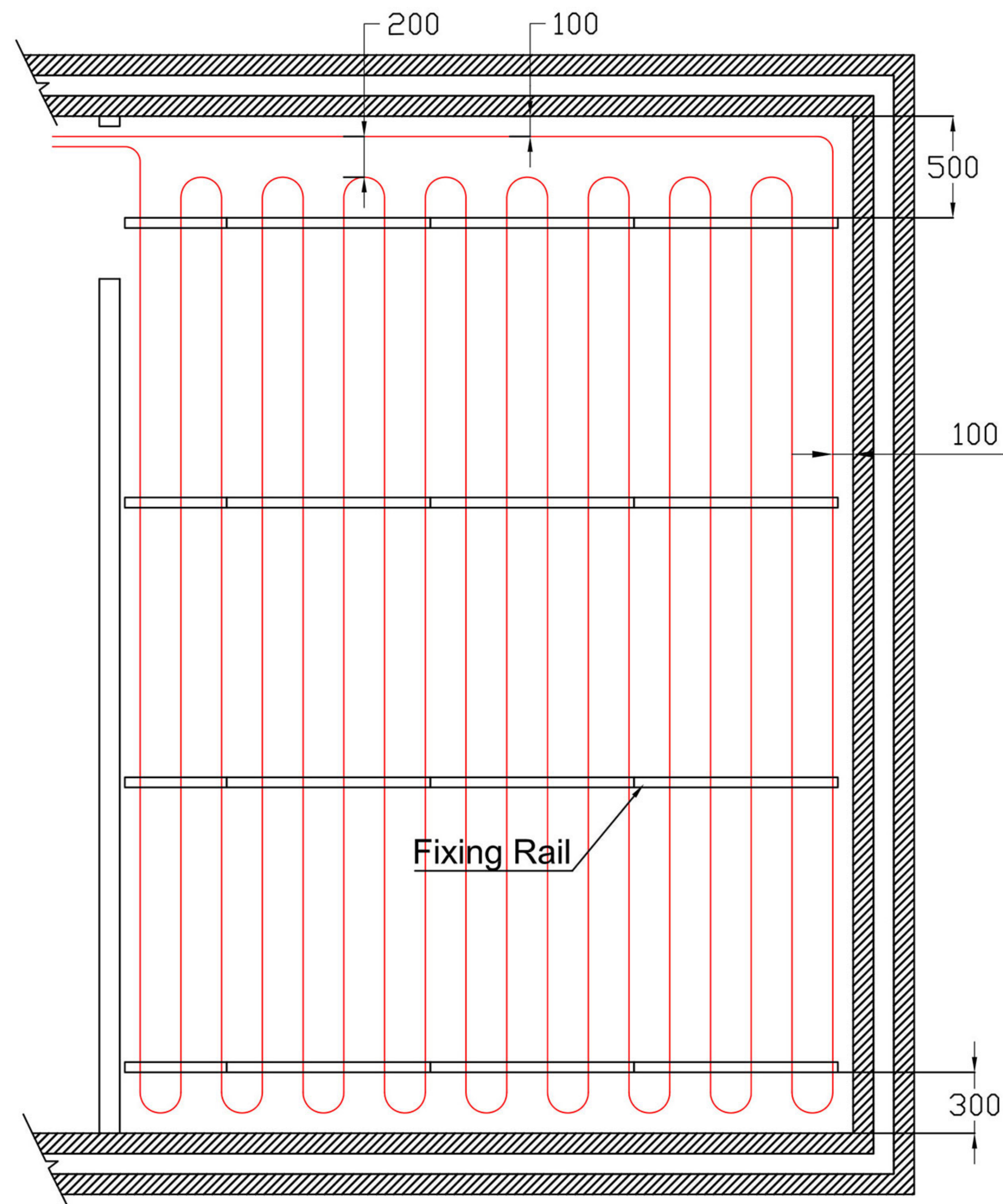
Typical Single Room Layout
