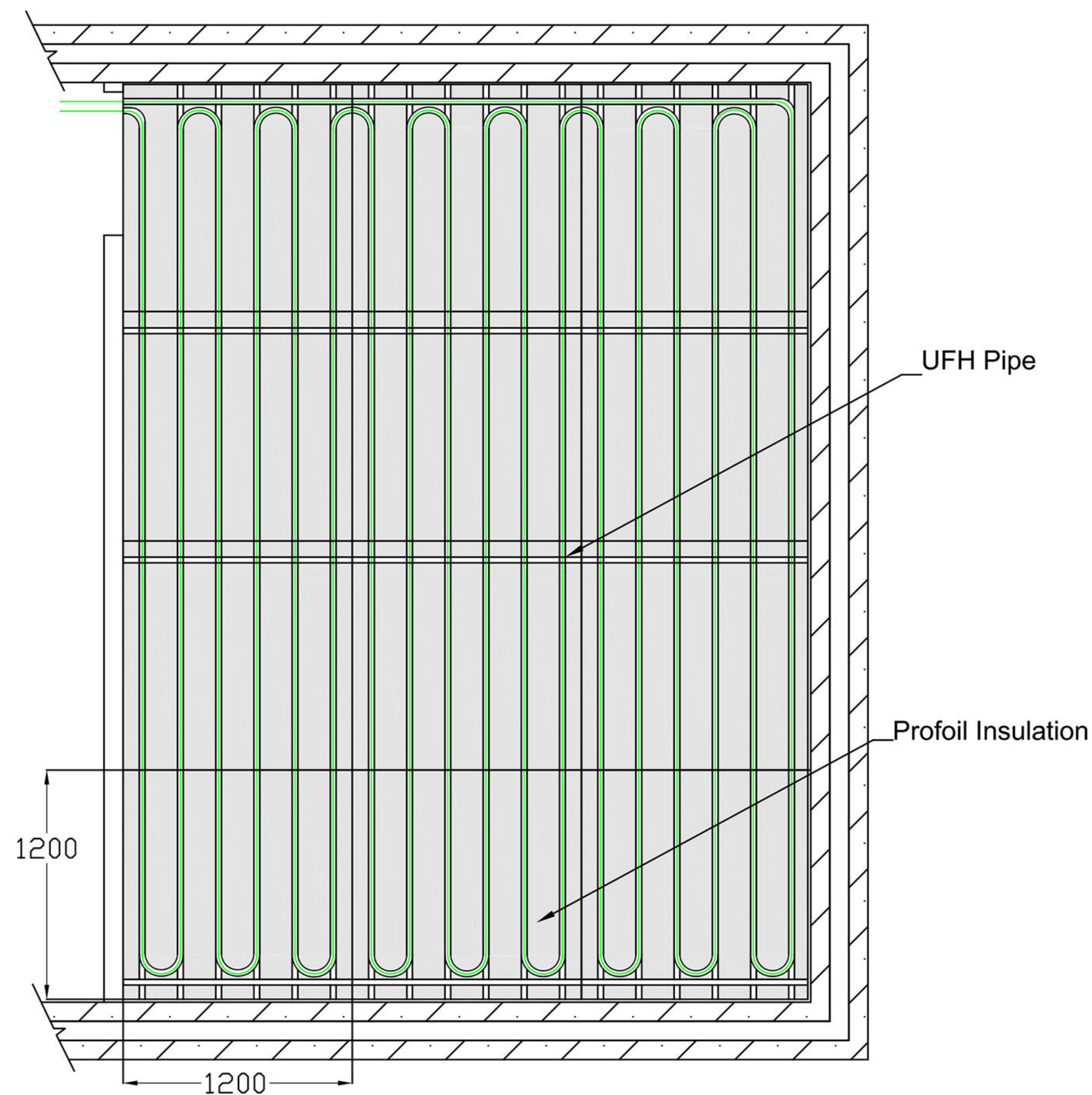
Typical Profoil 1200 x 1200mm Grooved Insulation Boards
