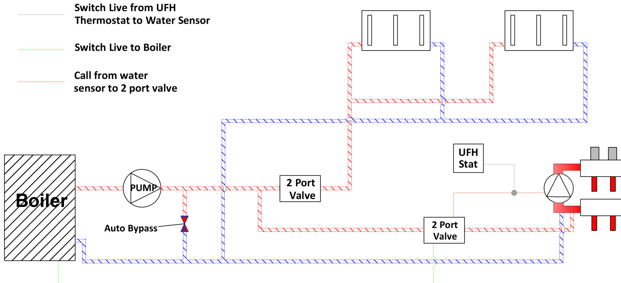
Schematic Plumbing Diagram Single Zone S Plan Combi Boiler
